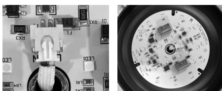
2-pin connector
