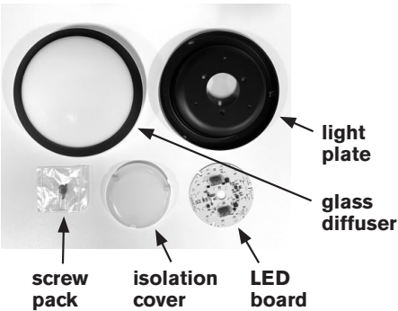
Optional Light Kit parts:
